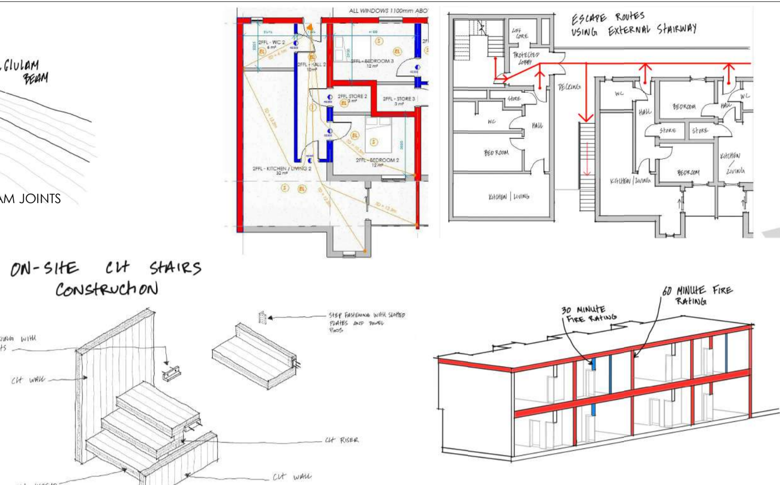
P1.2 INVESTIGATION INTO CLT STAIRS
